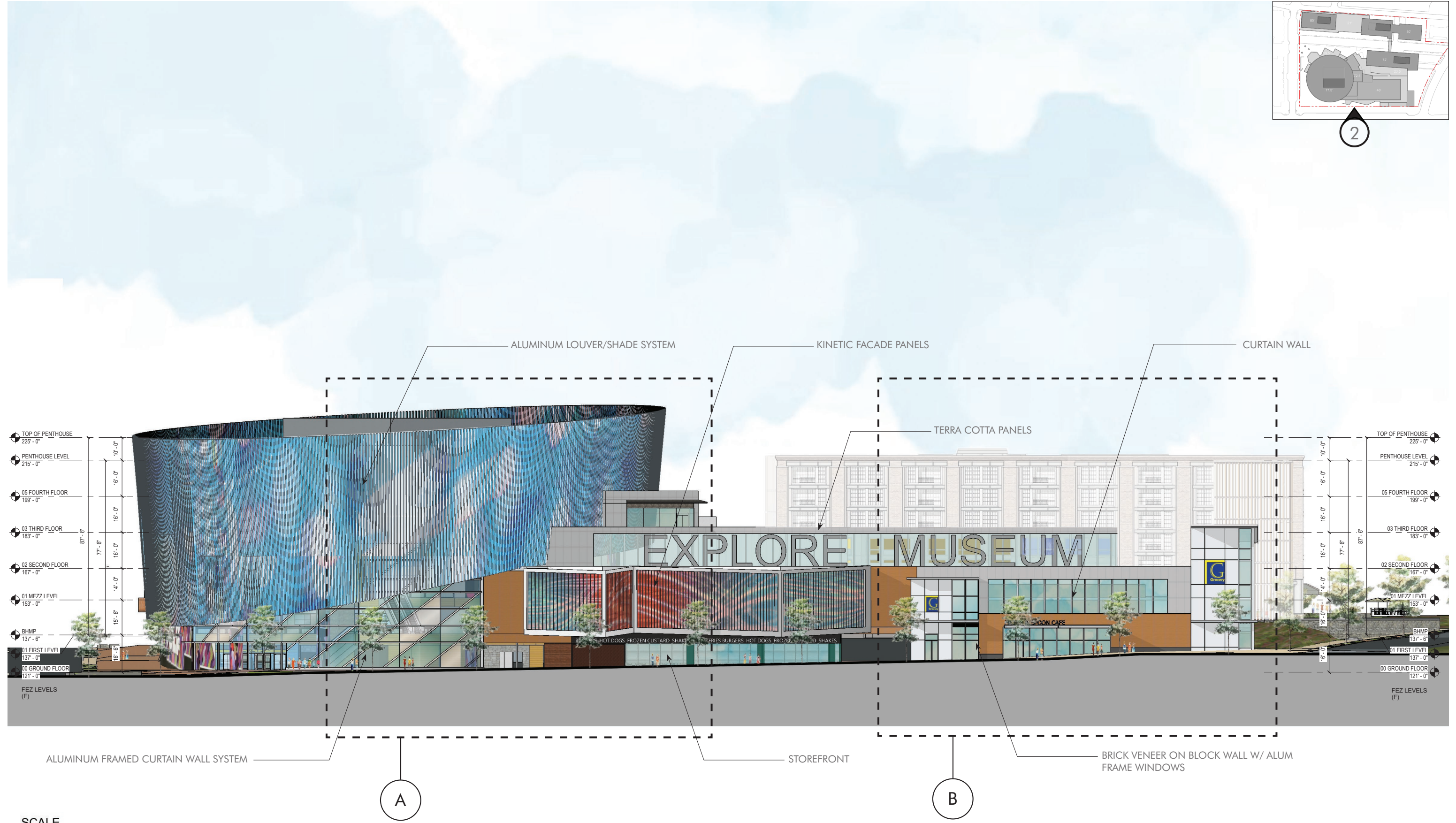
BUILDING ELEVATIONS & MATERIALS: SOUTH DAKOTA AVE NE ART PLACE AT FORT TOTTEN 60
